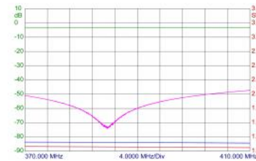
TYPICAL RESPONSE CURVE SWR 1
