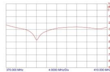
TYPICAL RESPONSE CURVE ANTENNA MUMOUNTING DETAILS 3-BZ/TETRA/I (with 1.5 m cable)
